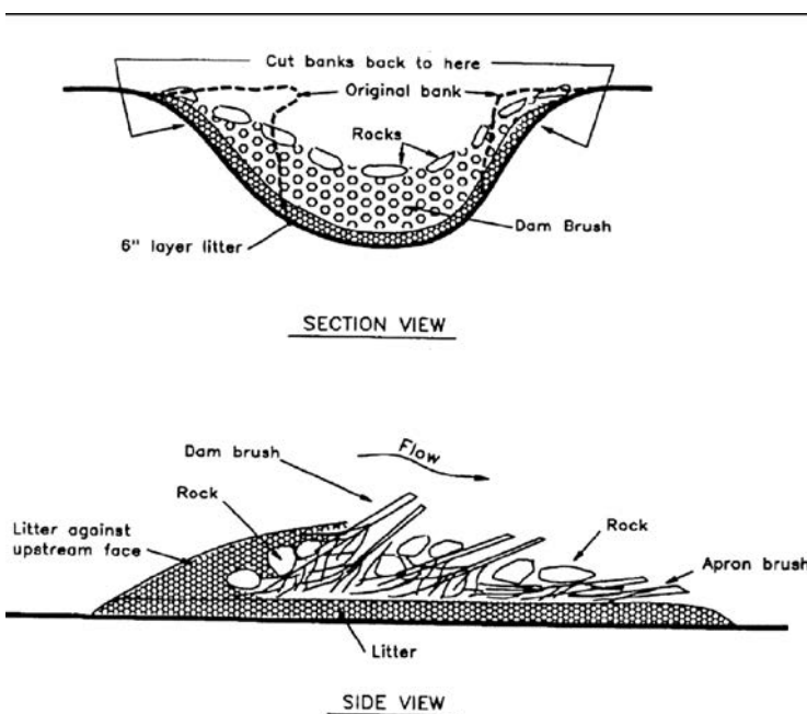
Figure 5. Brush and rock dam. Image courtesy of the California Department of Fish and Game.
