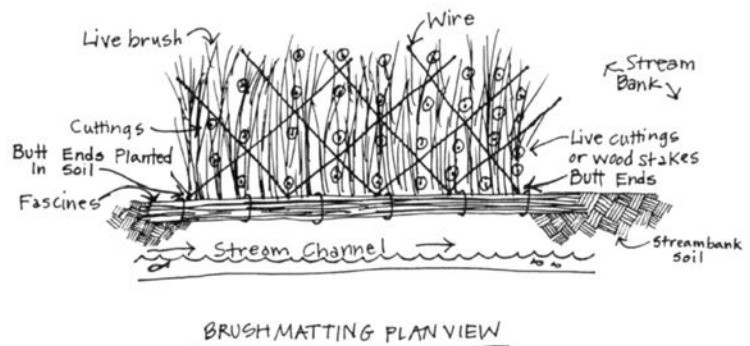
Figure 17. Brush matting slope protection. Image from Restoring Streams in Cities by Ann L. Riley. Excerpted by permission of Island Press, Washington D.C.
