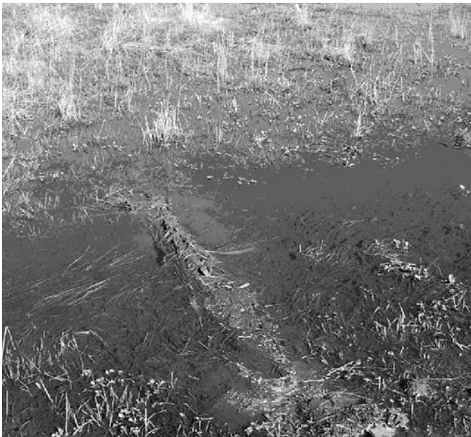
Figure 10. Bundle of cottonwood cuttings placed in a small ditch to slow run off and ultimately generate riparian vegetation through hardwood cutting. Photo by Rick Barney, NRCS
