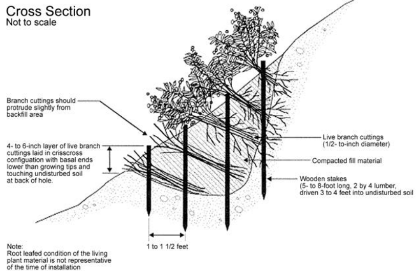
Figure 16. Branch-packing. Image from the USDA NRCS Engineering Field Handbook.
