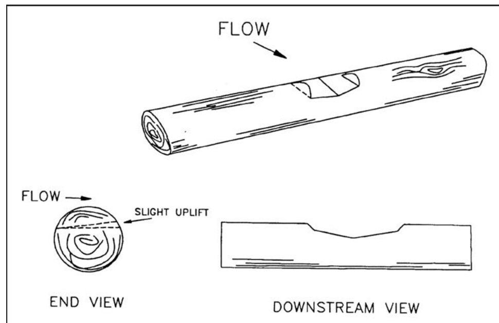
Figure 3. Notched log weir.
