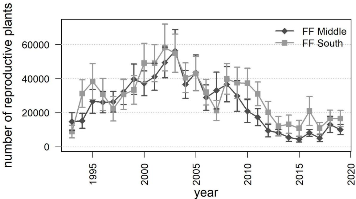
Figure 13. The total number of reproductive Lomatium cookii at Middle and South French Flat, 1993-2019. Error bars represent a 95% confidence interval.
