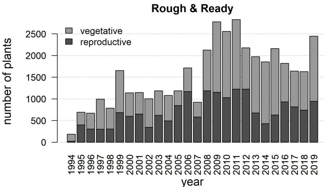
Figure 16. Population trends and the total number of plants (reproductive and vegetative) at Rough and Ready Creek, 1994-2019. There were only 26 reproductive plants recorded in 1994.
