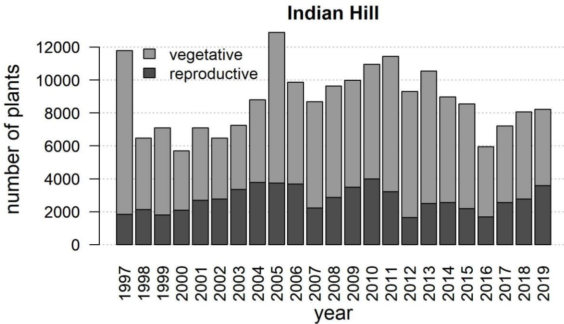
Figure 18. Number of vegetative and reproductive plants at Indian Hill, 1997-2019.
