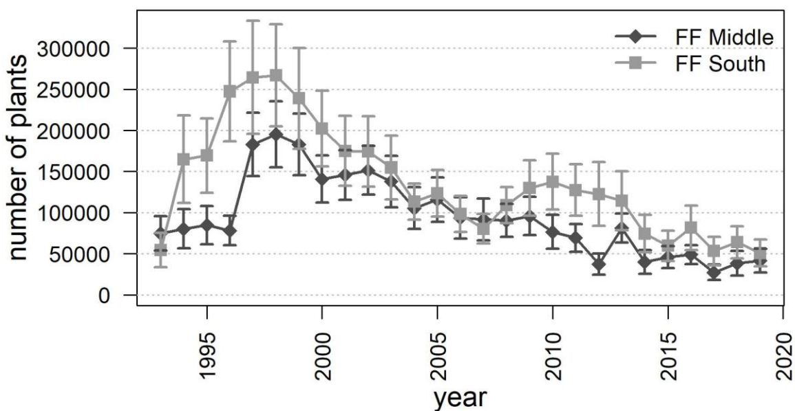
Figure 12. The total number of Lomatium cookii at Middle and South French Flat, 1993-2019. Error bars represent a 95% confidence interval.
