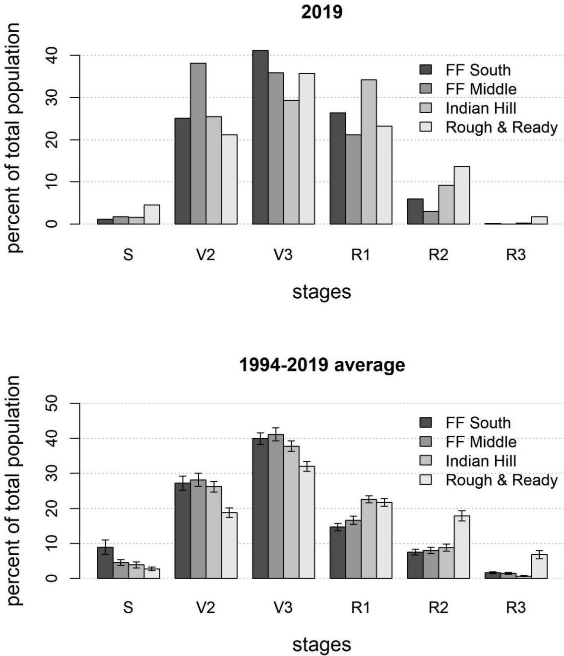
Figure 15. Lomatium cookii population structure in 2019 (top) and averaged over the course of the study (bottom) for the Middle French Flat subpopulation (1994-2019), South French Flat subpopulation (1994-2019), Rough and Ready Creek (1995-2019), and Indian Hill (1997-2019). Bars indicate the mean percentage of plants in each stage. Error bars in the lower graph represent +1 SE. See text for explanation of life-history stages.
