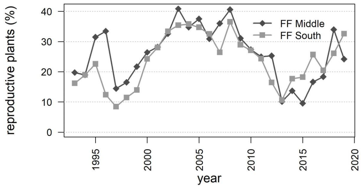
Figure 14. The number of reproductive Lomatium cookii relative to the total subpopulation at Middle and South French Flat, 1993-2019.
