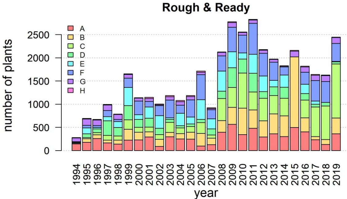
Figure 17. Population fluctuations in L. cookii patches A-H at Rough and Ready Creek, 1994-2019. Patches B-F were combined in 2015 and patches E-F were combined in 2018.
