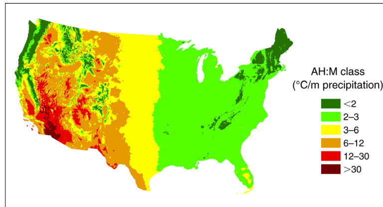
FIG. 2. Annual heat : moisture (AH:M) index class bands. AH:M was calculated as mean annual temperature (MAT, °C) plus 15°C (to obtain positive values) divided by mean annual precipitation in meters (Hamann and Wang 2005).
